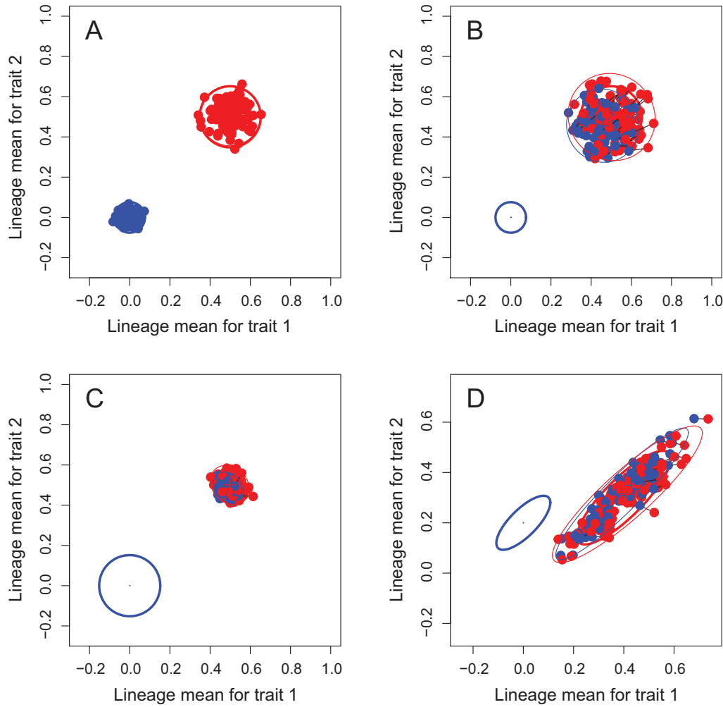
Figure 4: Sexual selection exaggerates the evolution of ornaments and mating preferences, producing a phenotypic tango (illustrated with sets of 100 lineages at generation 500; N_e = 5,000 ; P_{ii} = Q_{ii} = 1 ; G_{ii} = H_{ii} = 0.4 ; B_{ii} = 0.24 ; \nu_{ii} = 0.4 ; \nu_{ij} = 0 ). The 95% confidence ellipses for diversification of ornaments and preferences by natural selection alone are shown as light blue and red ellipses, respectively. The 95% confidence ellipses for the sample of ornament and preference means are shown as heavy blue and red ellipses, respectively. A , Evolution of ornaments and preferences in the absence of sexual selection ( \omega_z = 4, 0, 0, 4 ; \omega_y = 19, 0, 0, 19 ; \theta_z = 0, 0 ; \theta_y = 0.5, 0.5 ; B_{ii} = 0 ). B , The evolution of ornaments and preferences in the presence of sexual selection is a tango ( \omega_z = 4, 0, 0, 4 ; \omega_y = 19, 0, 0, 19 ; \theta_z = 0, 0 ; \theta_y = 0.5, 0.5 ; B_{ii} = 0.24 ). The positions of ornament and preference means for a particular lineage are shown as blue and red dots, respectively, connected by a black line. C , When stabilizing selection on ornaments and preferences is reversed (weak on ornaments, strong on preferences), extraordinary evolution of ornaments is eliminated ( \omega_z = 19, 0, 0, 19 ; \omega_y = 4, 0, 0, 4 ; \theta_z = 0, 0 ; \theta_y = 0.5, 0.5 ; B_{ii} = 0.24 ). D , Correlational natural selection on ornament and preference changes their 95% confidence ellipses from circles to inclined ellipses ( \omega_z = 9, 7.5, 7.5, 9 ; \omega_y = 29, 25, 25, 29 ; \theta_z = 0, 0.2 ; \theta_y = 0.4, 0.3 ; B_{ii} = 0.24 ; \nu_{11} = \nu_{22} = 0.4 ; \nu_{12} = \nu_{21} = 0.3 ).
