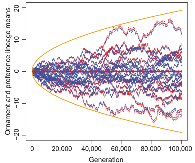
Figure 7: Simulated evolution of ornaments and preferences with a moving preference optimum (illustrated with a set of 25 lineages; N_e = 500 ; P_{ii} = Q_{ii} = 1 ; G_{ii} = H_{ii} = 0.4 ; B_{ii} = 0.24 ; \nu_{ii} = 0.4 ; \nu_{ij} = 0 ; \omega_z = 9, 0, 0, 9 ; \omega_y = 9,999, 0, 0, 9,999 ; \sigma_\theta^2 = 0.00055 ). Conventions are as in figure 6. The 95% confidence limits for ornament diversification by natural selection alone are not visible. The orange curve shows the 95% confidence limits for diversification of preference means evolving under a model in which the preference optimum moves by Brownian motion.
